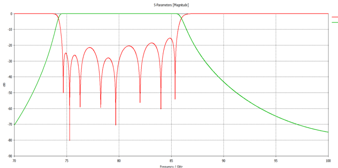
S21 vs Frequency
